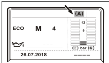
(A): Auxiliary brake engaged
